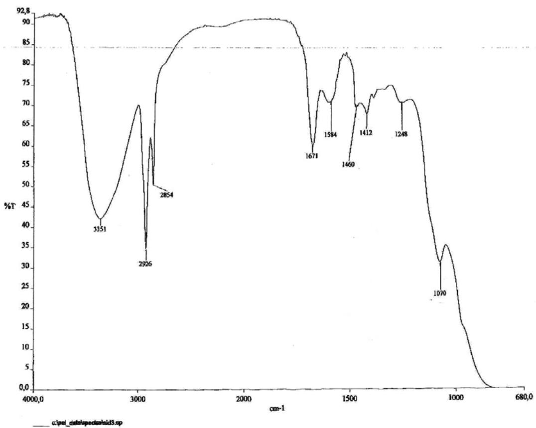
IR spectrum (film) of turbinamide
